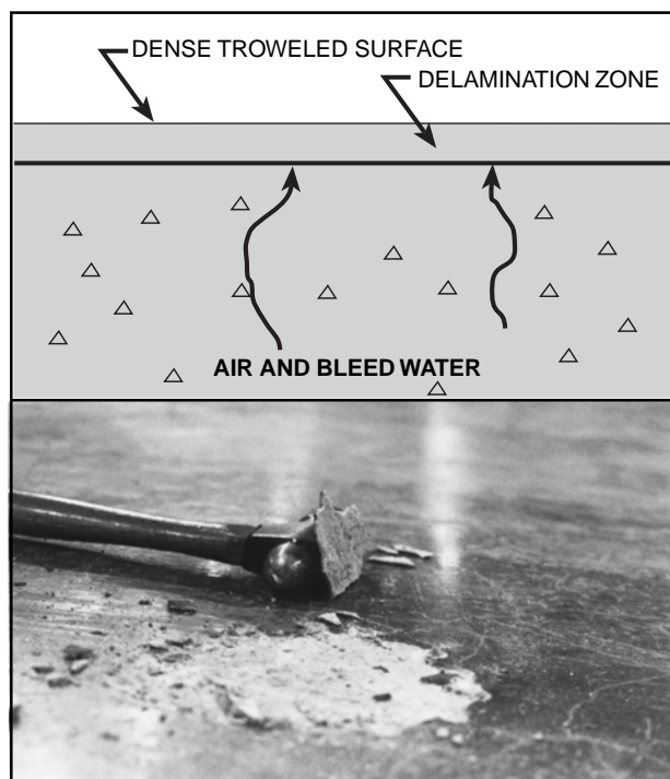
Delaminated Concrete
